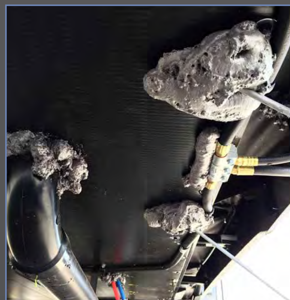
Forced Air, Heated and Enclosed Gate Valves and Underbelly
