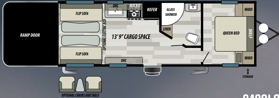
242SLC DRY WEIGHT 6,859 LBS
