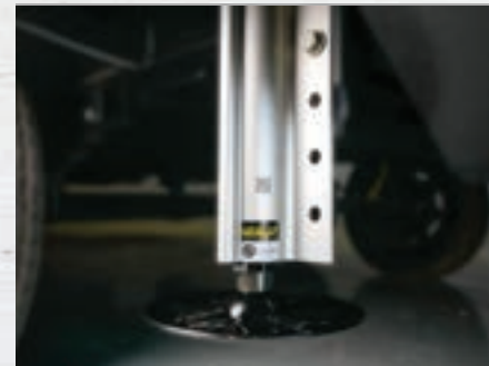
LEVELING SYSTEM The patented six-point "Level Up" hydraulic leveling system levels an RV in less than a minute using a one-touch auto-leveling feature and includes an auto re-hitch memory function that remembers the exact height at which the RV was unhitched.
