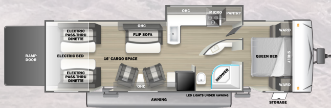
29RQMX/29KSGDX (16' CARGO)
