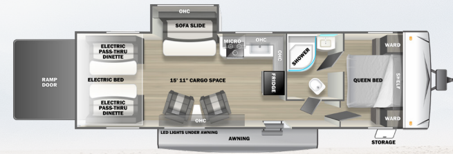
RQ2715 AVAILABLE AS FQ2715G (FIBERGLASS) (15' 11'' CARGO)
