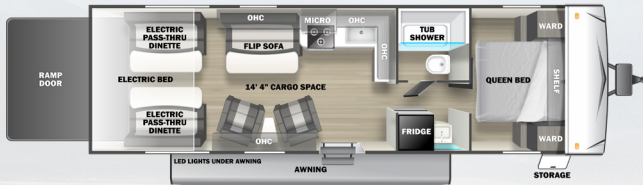
FQ2514 AVAILABLE AS FQ2514G (FIBERGLASS) (14' 4'' CARGO)
