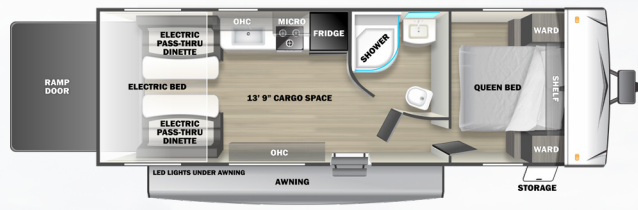
FQ2413 AVAILABLE AS FQ2413G (FIBERGLASS) (13' 9'' CARGO)
