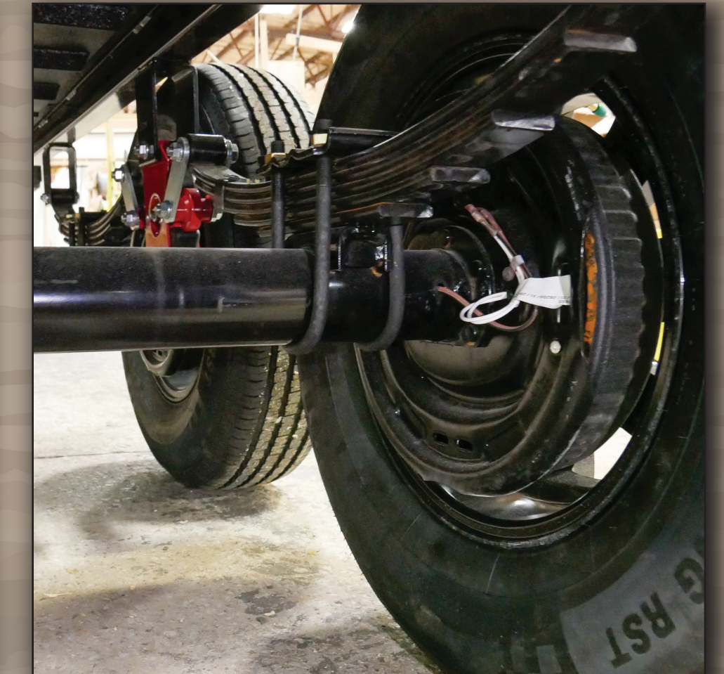
7K DEXTER EZ LUBE AXLES WITH NEVR-ADJUST BRAKES
