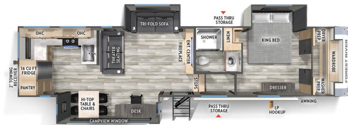
33CHEF HITCH: 1,885 GWR: 13,885 UWW: 10,558 CCC: 3,327 LENGTH: 38'3" HEIGHT: 13'3" WIDTH: 96" TANKS (F/B/G): 60 38 76 AWNINGS: 15' & 11'
